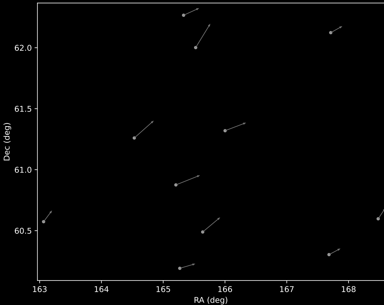
APOGEE DR17 Cluster 14 Proper Motion Vectors (n=11)
