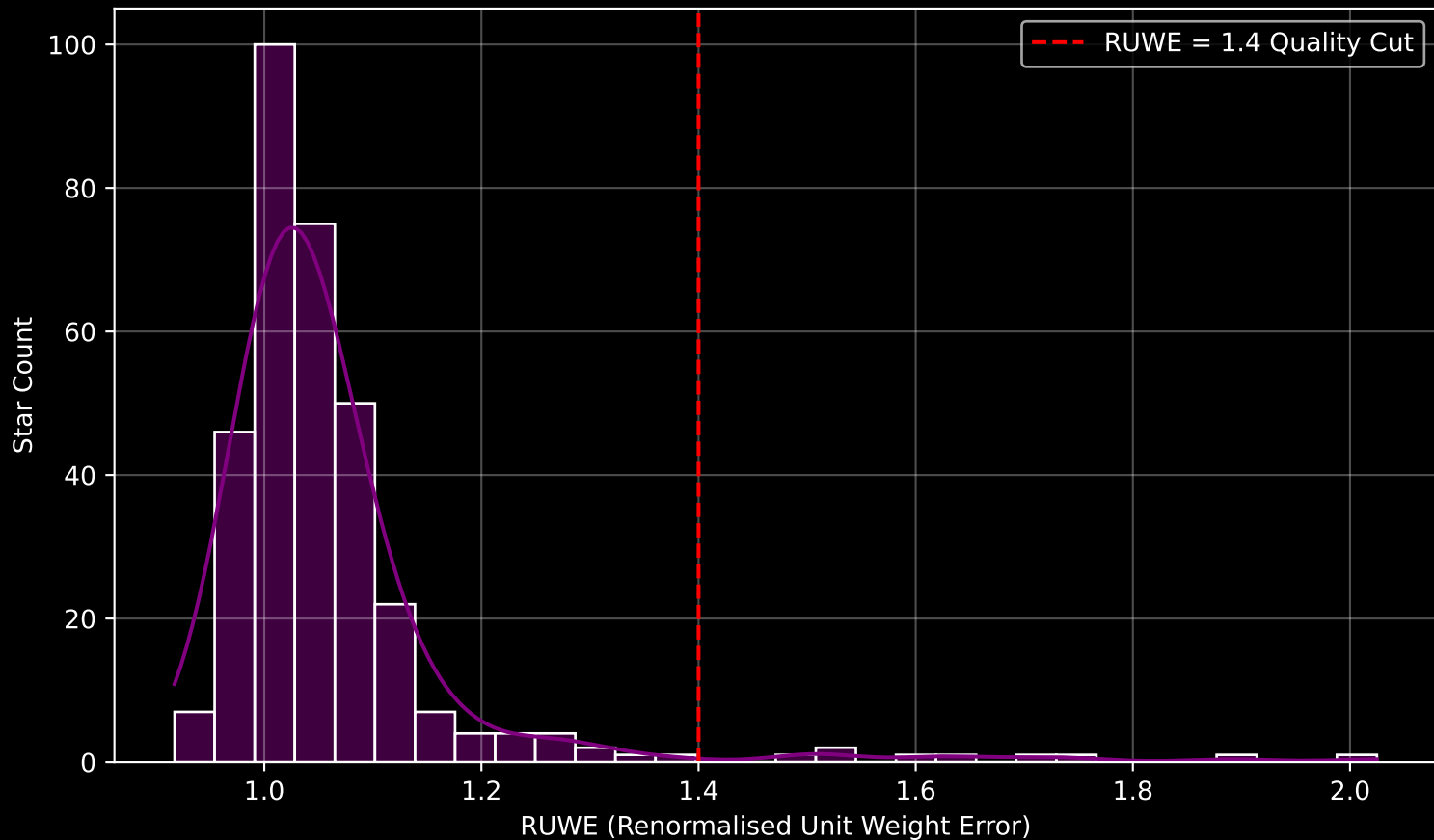
GAPOGEE DR17 Field [146+08] RUWE Distribution (n= 332)
