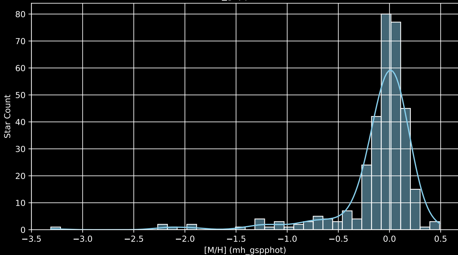
APOGEE DR17 Field: [146+08 [M/H] (mh_gspphot) (n= 331)
