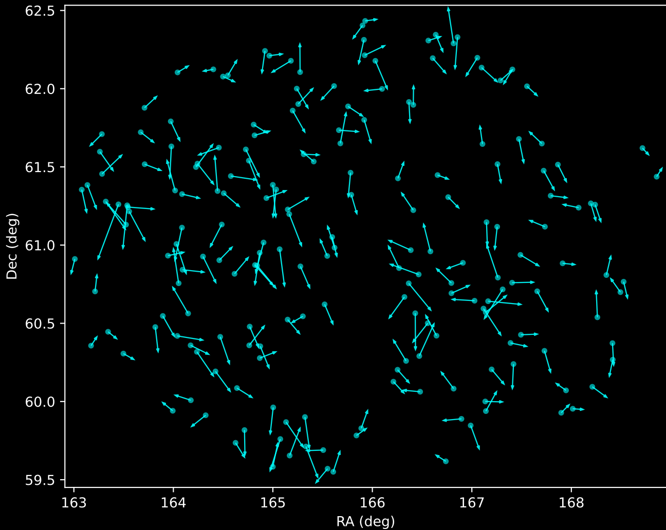
APOGEE DR17 Noise Stream Proper Motion Vectors (n=194)
