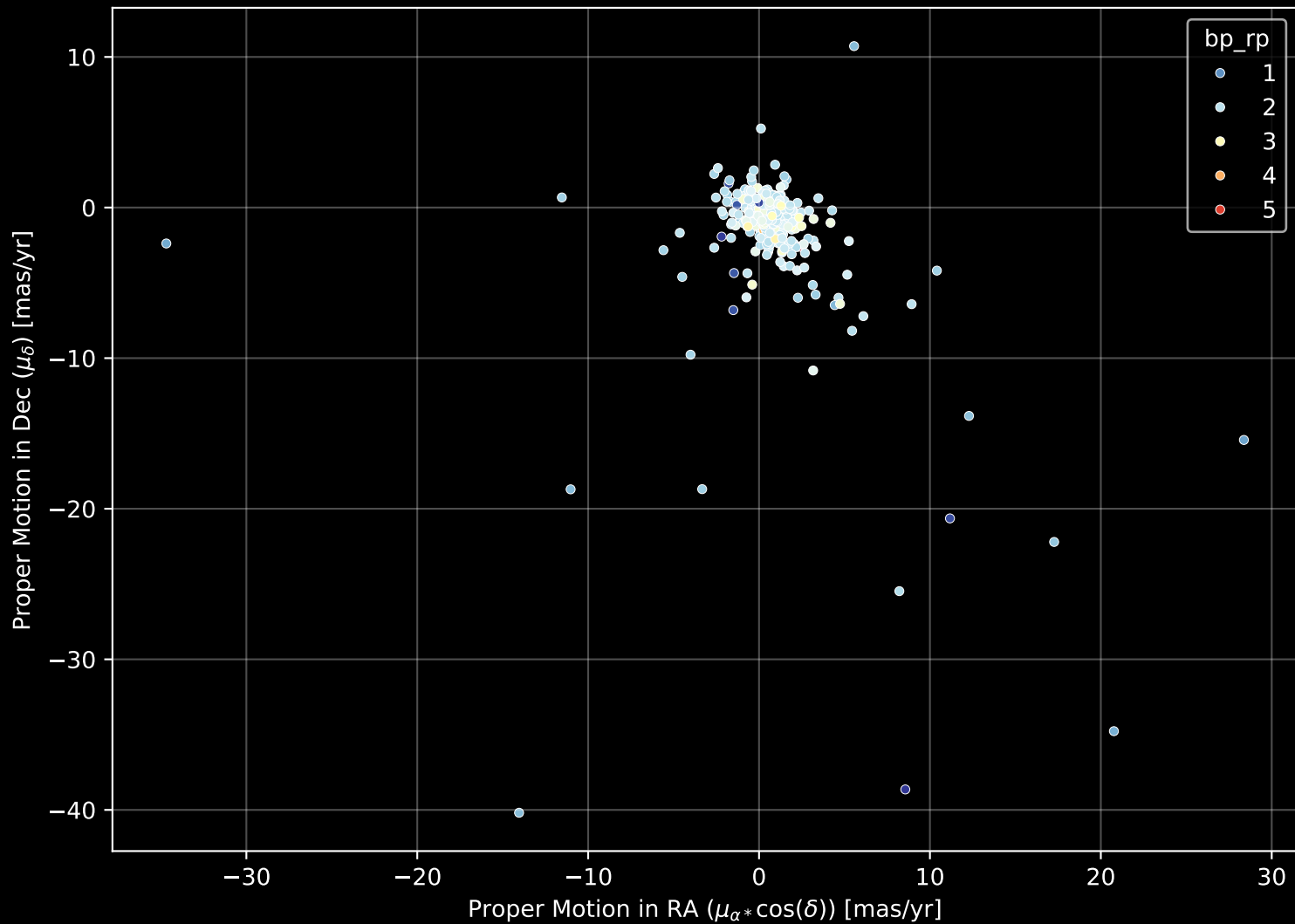
APOGEE DR17 Field: [146+08] Proper Motion Diagram (n= 333)
