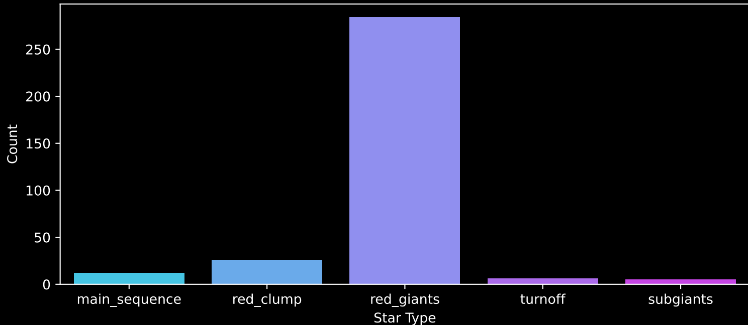
APOGEE DR17 Field: [146+08] Count plot of Star Type
