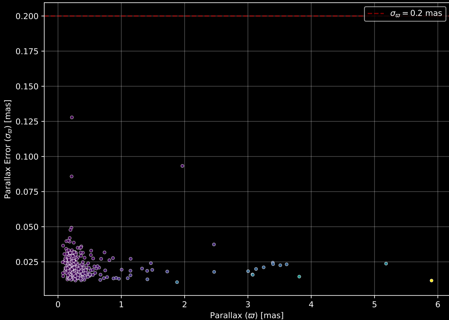
APOGEE DR17 Field: [146+08] Parallax Quality (n= 333)
