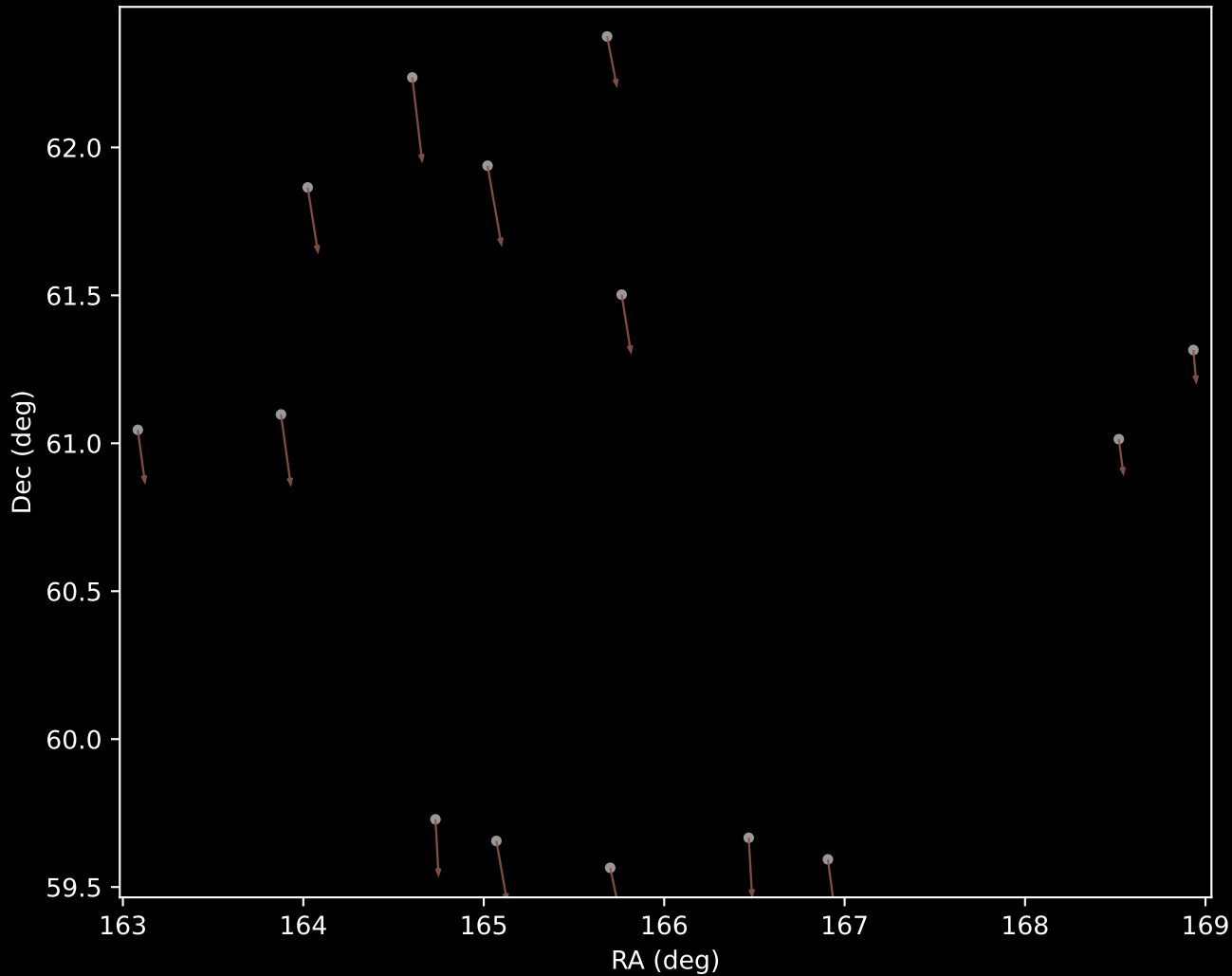
APOGEE DR17 Cluster 10 Proper Motion Vectors (n=14)
